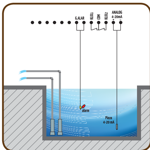
4-20mA meters
